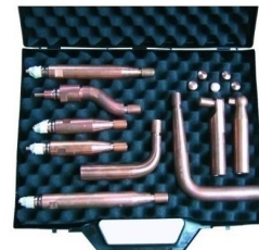
Accessories case, electrode set and 13 mm caps
