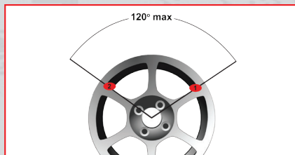
In split weight mode, adhesive weights can be hidden behind adjacent spokes of alloy rim
