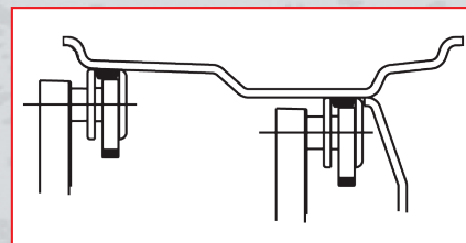
ALU 2P/3P mode for exact weight positioning
