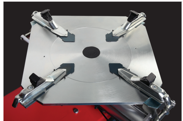
Center-clamp design with covered sliding grooves ensure operator safety
